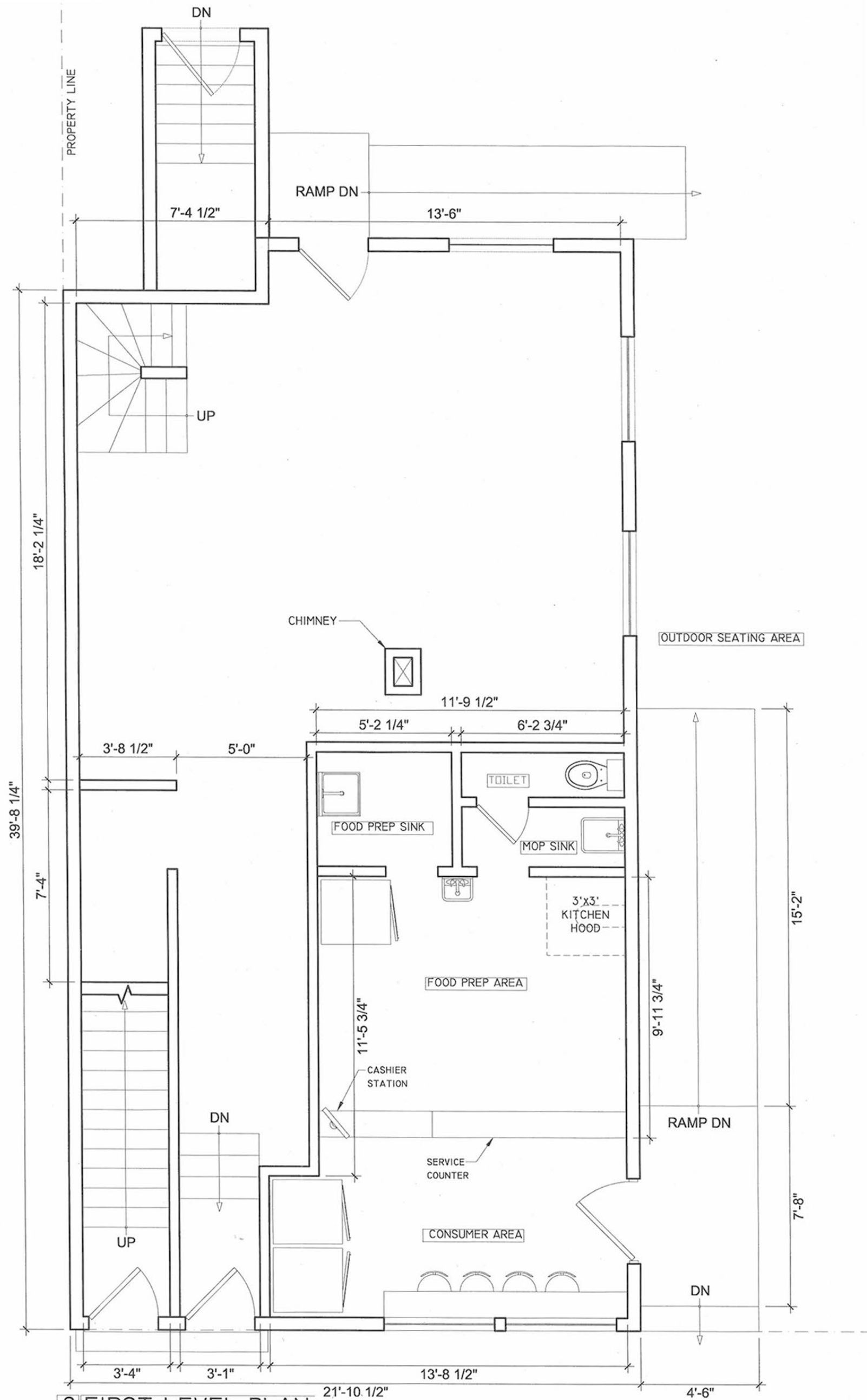
2 FIRST LEVEL PLAN
