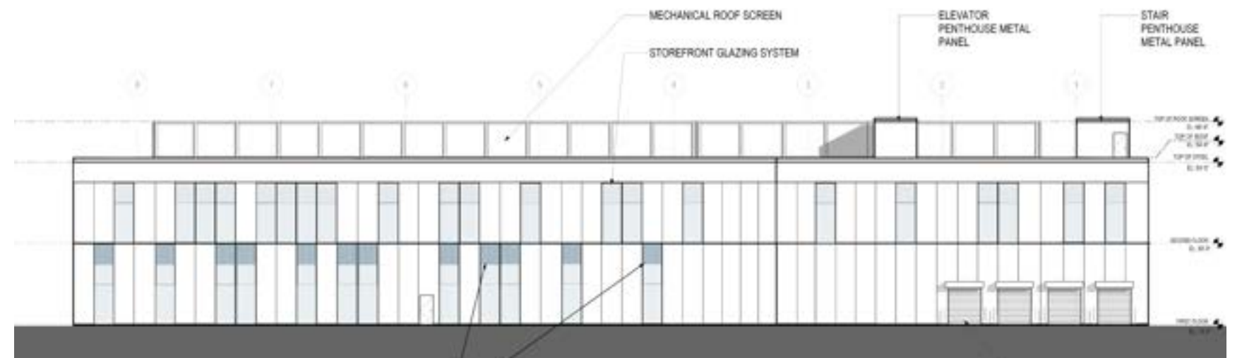
NORTH ELEVATION
