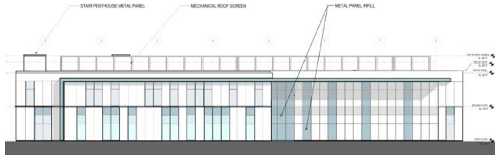
SOUTH ELEVATION
